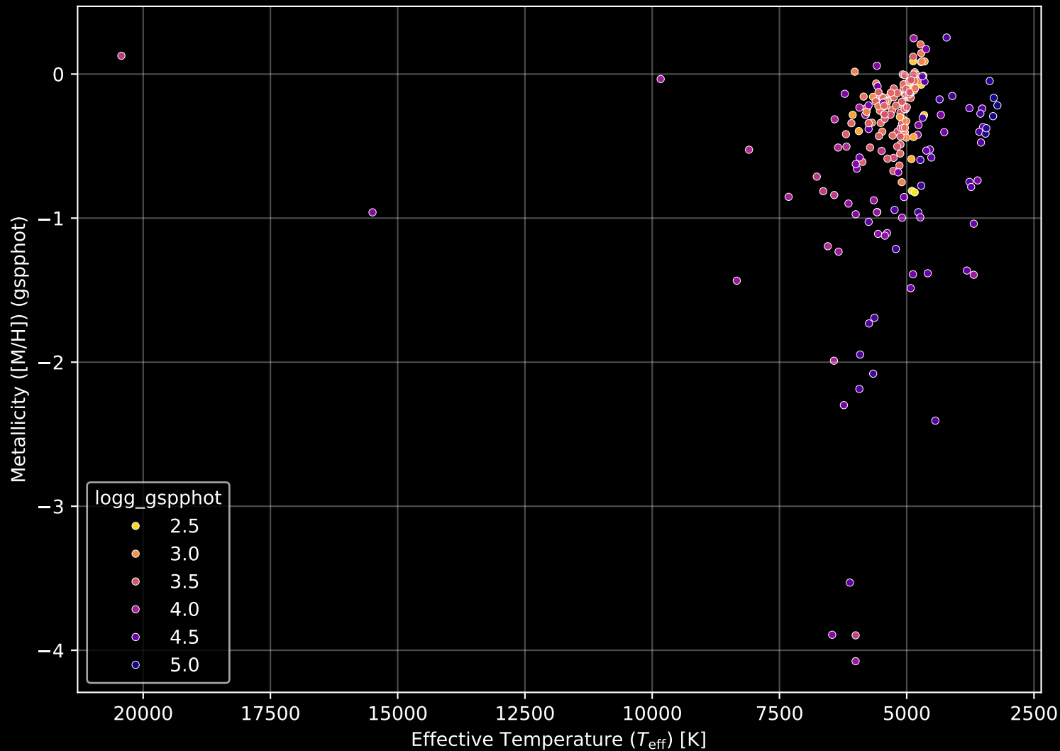
APOGEE DR17 Field: [K2_C11_359+13_btx] Stellar Population Parameters (n= 213)
