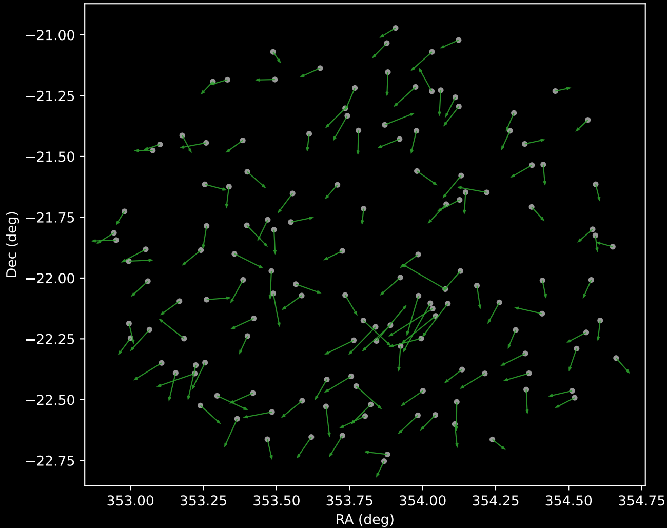
APOGEE DR17 Cluster 4 Proper Motion Vectors (n=141)
