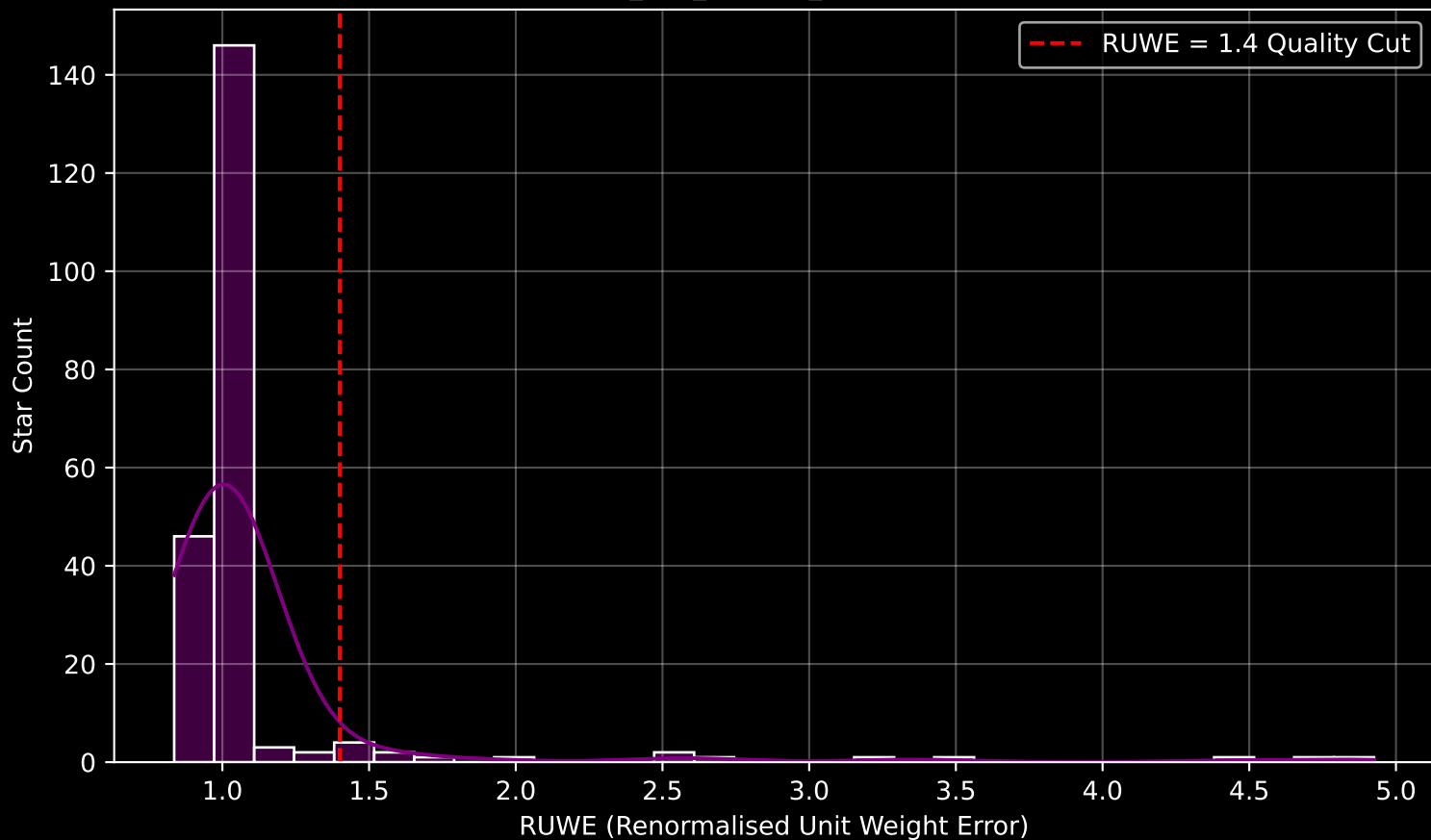
GAPOGEE DR17 Field [K2_C11_359+13_btx] RUWE Distribution (n= 213)
