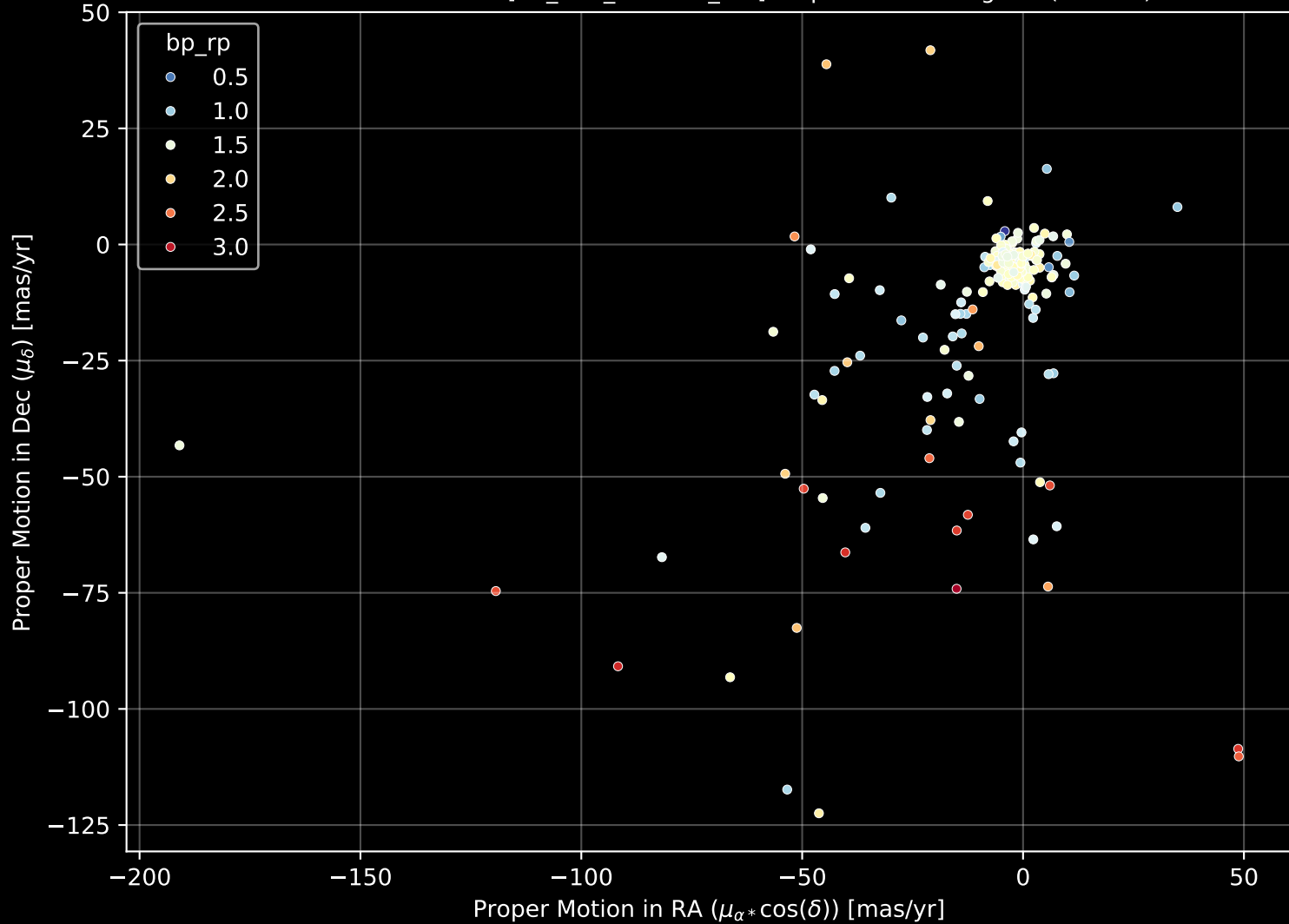
APOGEE DR17 Field: [K2_C11_359+13_btx] Proper Motion Diagram (n= 213)
