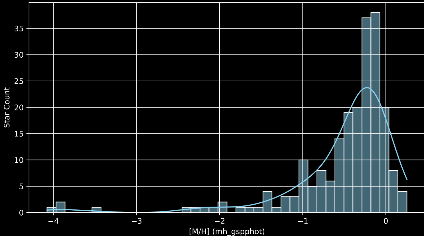
APOGEE DR17 Field: [K2_C11_359+13_btx [M/H] (mh_gspphot) (n= 213)
