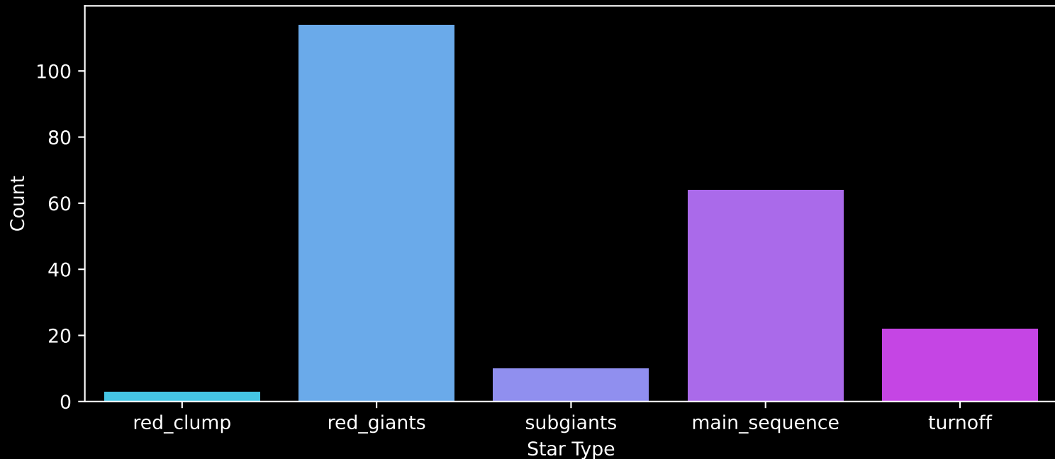
APOGEE DR17 Field: [K2_C11_359+13_btx] Count plot of Star Type
