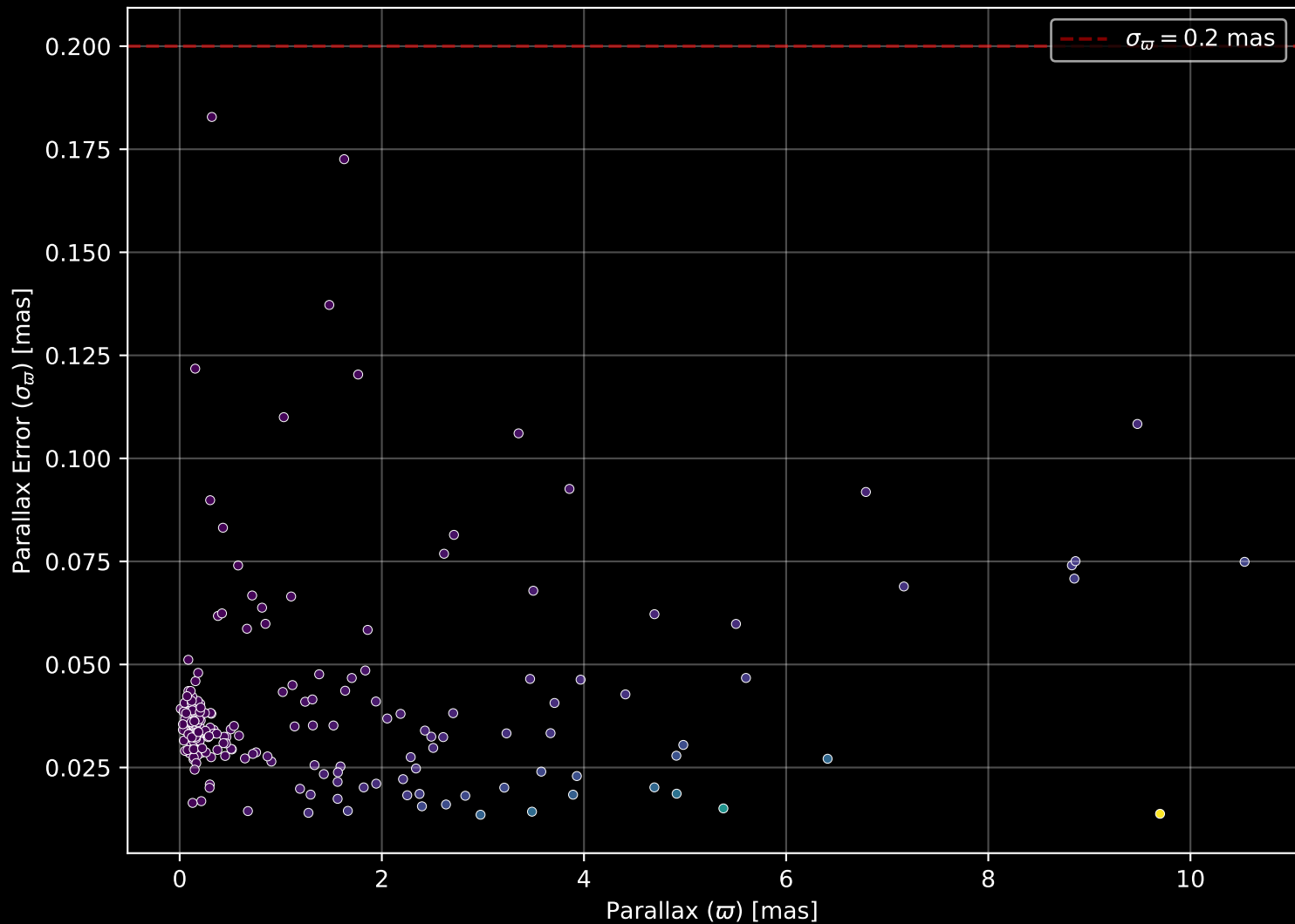
APOGEE DR17 Field: [K2_C11_359+13_btx] Parallax Quality (n= 213)
